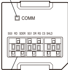
RS232C terminal block
